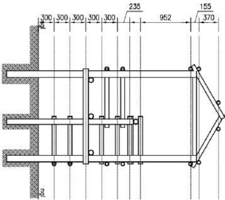
WEST ELEVATION scale 1:50
